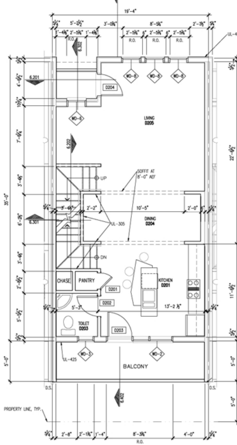
2.102 SECOND FLOOR PLAN
