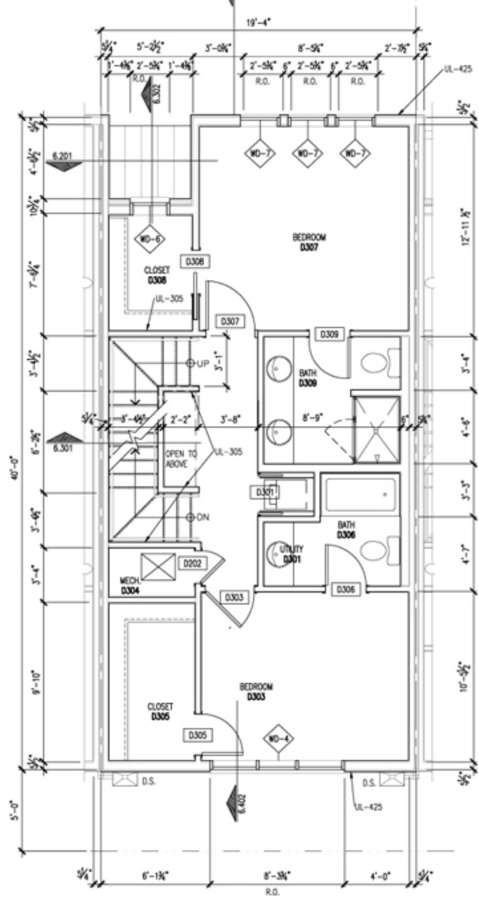
2.103 THIRD FLOOR PLAN
