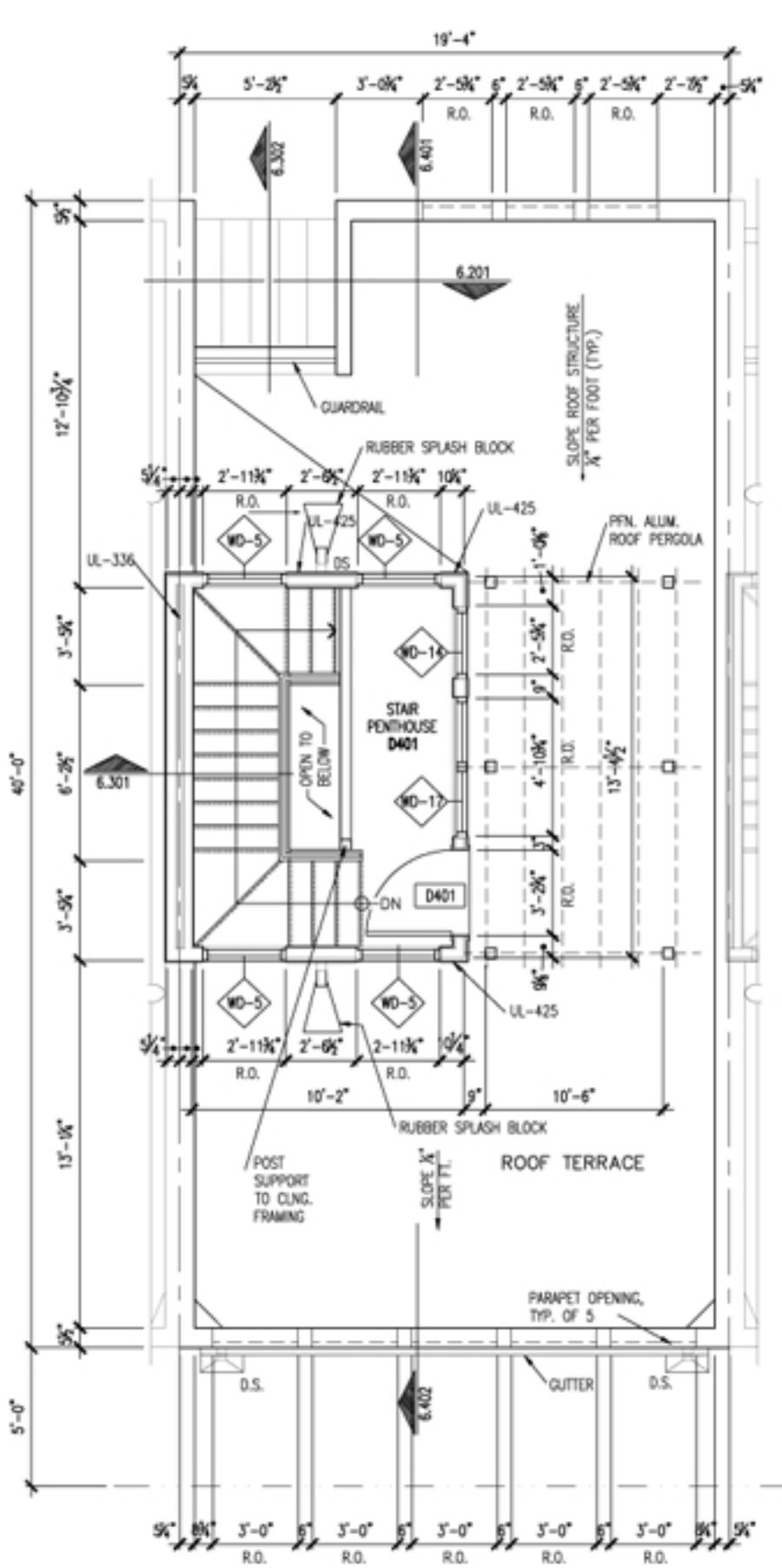
2.104 ROOF TERRACE PLAN
