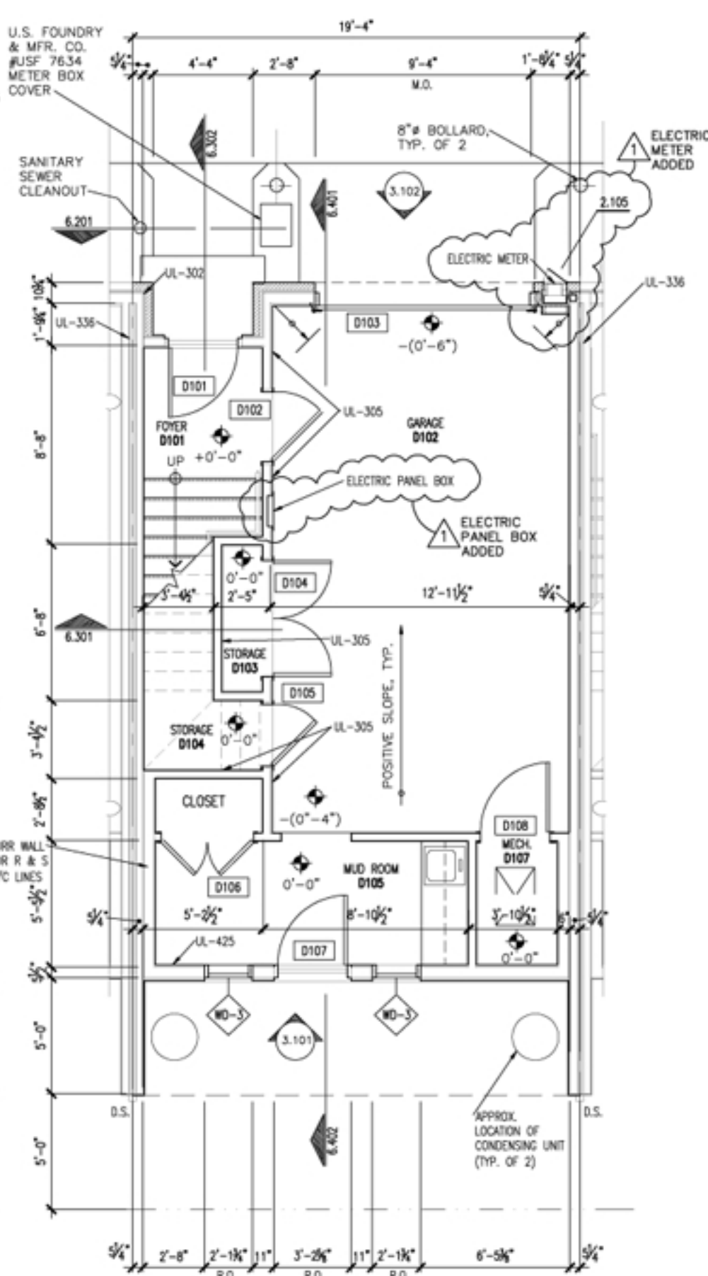
2.101 FIRST FLOOR PLAN
